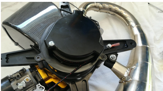
Easy-Starter before modification
